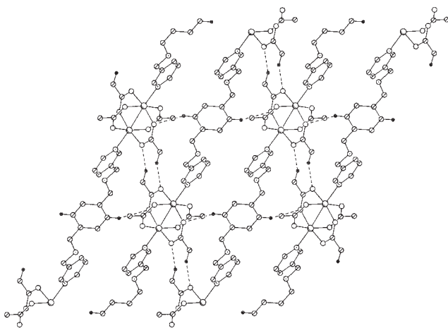
Fig. 4. 2D network structure of complex 2 with hydrogen bonds indicated by the dashed lines.
