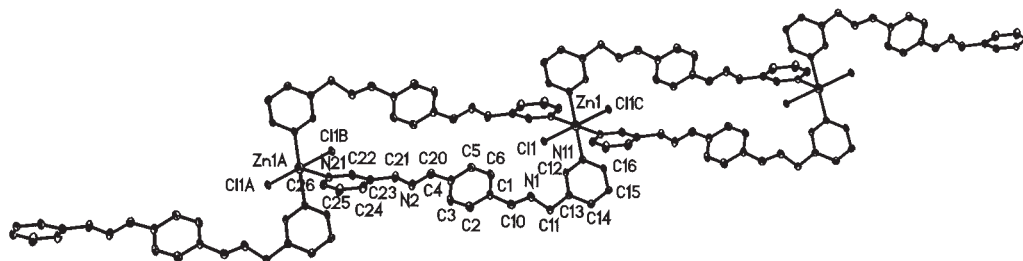
Fig. 5. Atomic displacement ellipsoid drawing (50% probability level) and atomic labeling system for the complex 3 . Hydrogen atoms are omitted for clarity.
