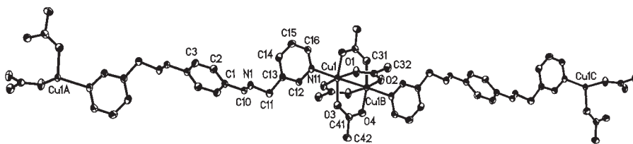
Fig. 3. Crystal structure of complex 2 with the thermal ellipsoids drawn at 50% probability level. Hydrogen atoms are omitted for clarity.
