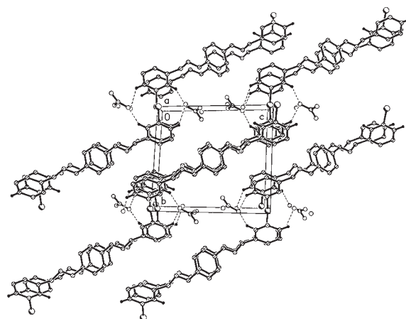
Fig. 2. Crystal packing diagram of complex 1 on bc plane with hydrogen bonds indicated by dashed lines.
