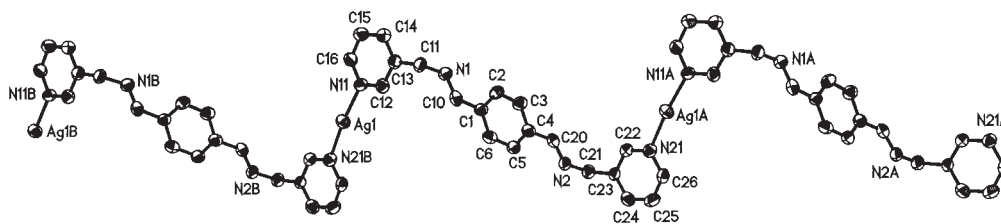
Fig. 1. Infinite 1D zigzag chain structure (cation part) of 1 . The anions, solvents and hydrogen atoms are omitted for clarity, and the thermal ellipsoids are drawn at 50% probability level.
