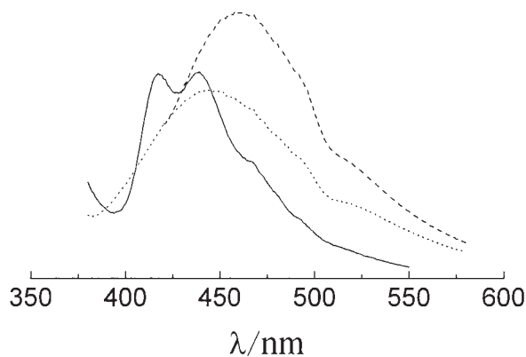
Fig. 8. Photo-induced emission spectrum of 2 with \lambda_{\text{ex}} = 360 nm (—) and photo-induced emission spectrum of 3 with \lambda_{\text{ex}} = 364 nm (---) and \lambda_{\text{ex}} = 398 nm (···) in the solid state at room temperature.
