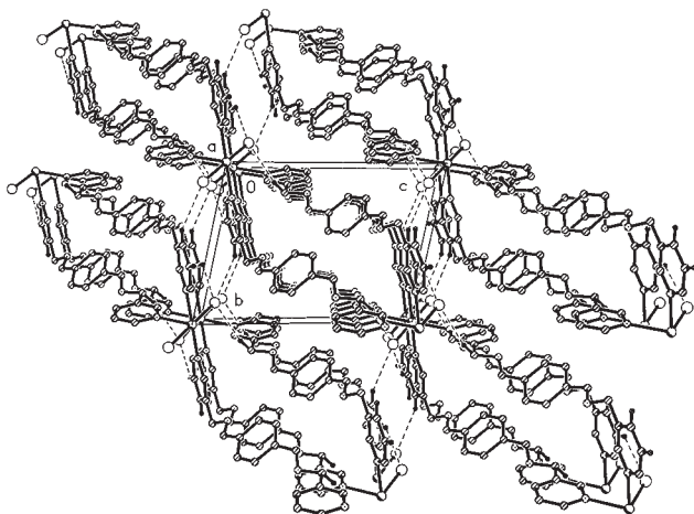
Fig. 6. 3D structure of 3 linked by C–H...Cl hydrogen bonds indicated by the dashed lines.
